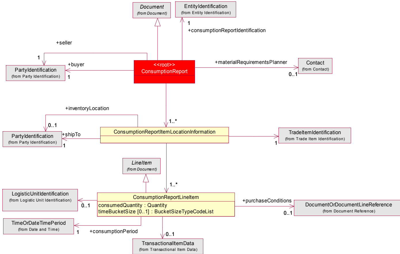
Figure 2 – Class Diagram: Business Document
