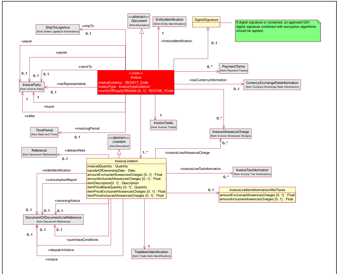
Figure 5-1 Class Diagram Invoice
