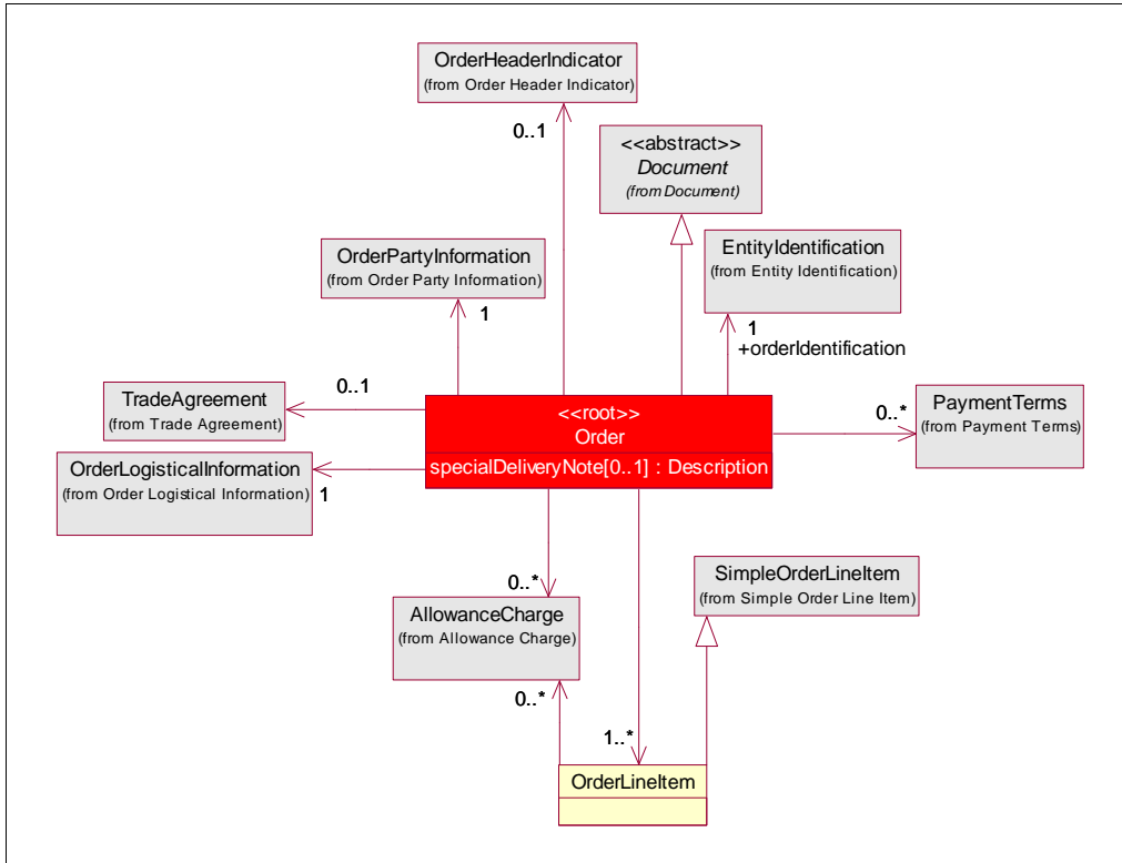
Figure 5-1 Class Diagram: Order
