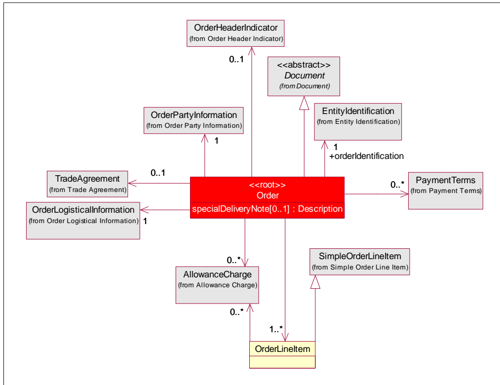
Figure 5-1 Class Diagram: Order
