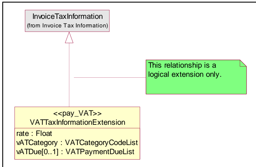
Figure 5-4 Class Diagram VAT Tax Information Extension
