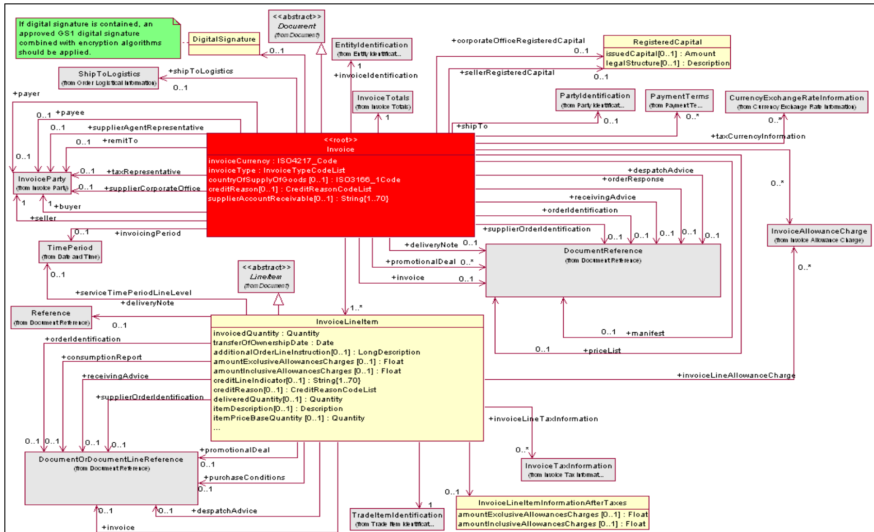
Figure 5-1 Class Diagram Invoice
